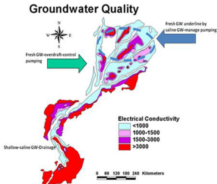
Figure 6: Three distinct groundwater zones of the Indus Basin of Pakistan
