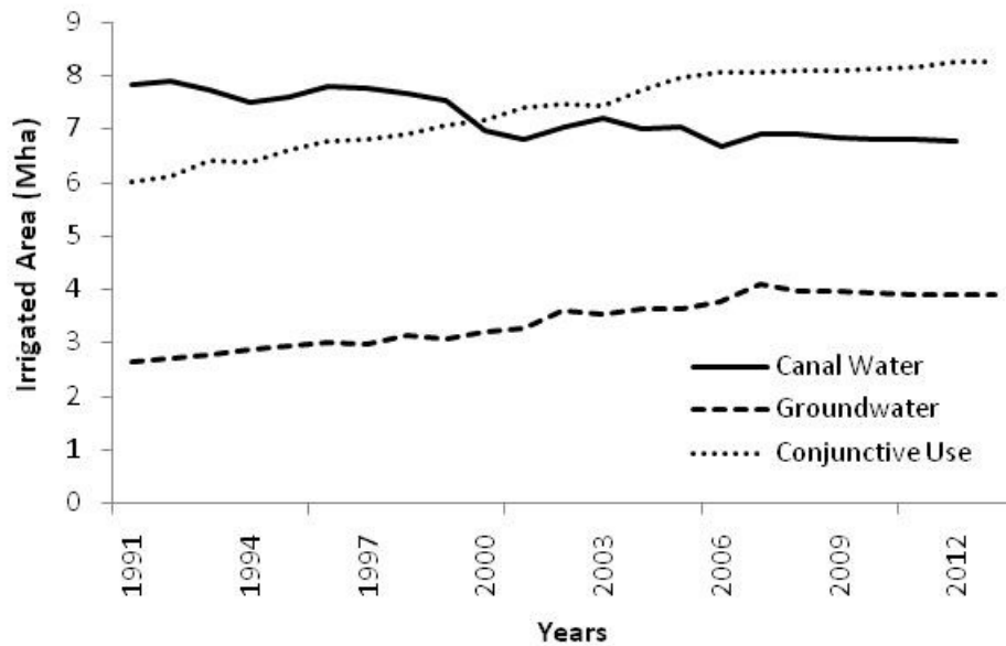
Figure 7: Trends of different modes of irrigation in the Punjab Province of Pakistan
